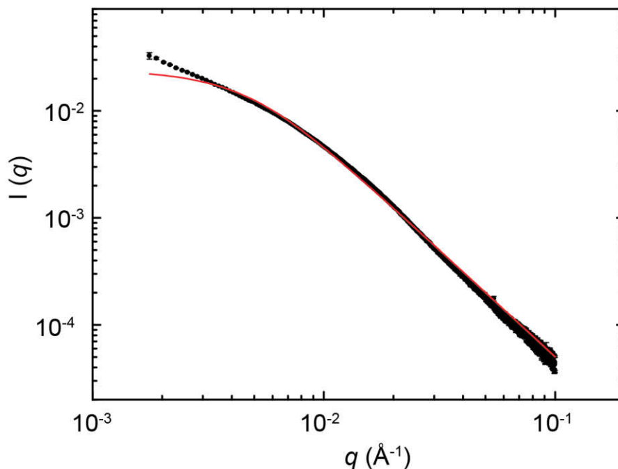
Figure S2. SAXS pattern of an equimolar ( 1.0 \times 10^{-3} \text{ M} ) mixture of CB[8] and 2 in D 2 O after incubation. The continuous curve is a least squares fit to the Gaussian chain model with a mean R_g of 31 nm. At high values of q (i.e. q \times R_g \gg 1 ) the Debye scattering function scales with q^{-2} .
