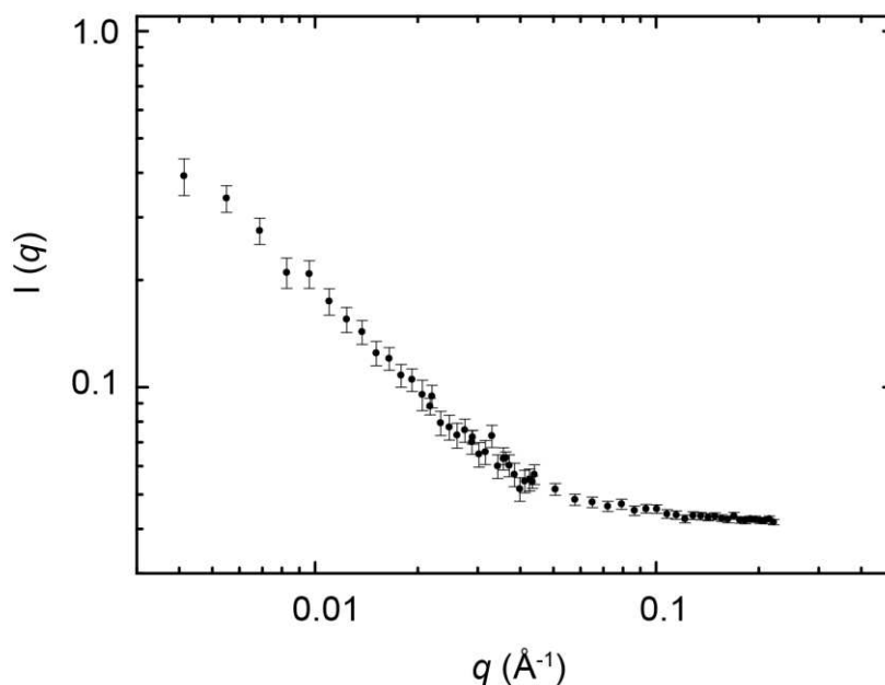
Figure S8. SANS pattern of an equimolar ( 1.0 \times 10^{-3} \text{ M} ) mixture of CB[8] and 2 in \text{D}_2\text{O} .
