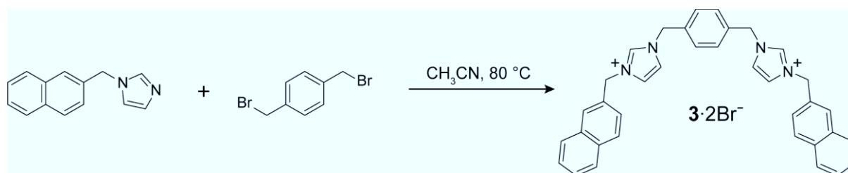
Scheme S1. Synthesis of guest molecule 3 .
