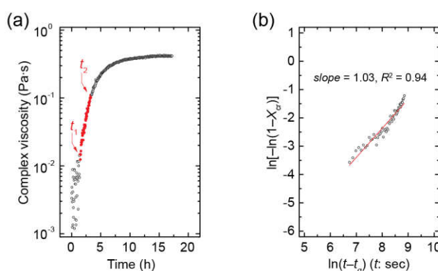
Figure S27. Dependence of \eta^* as a function of time (a) for an aqueous equimolar mixture of 3 and CB[8] ( 1.0 \times 10^{-3} M, H 2 O, 293 K) and corresponding Avrami plot (b).
