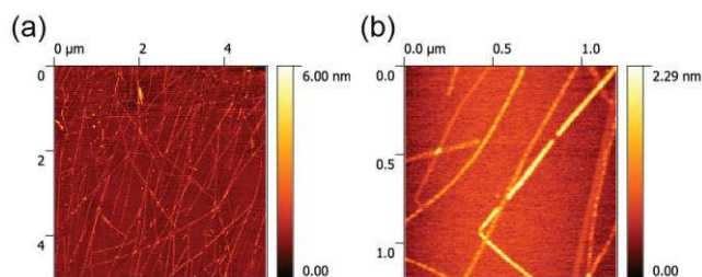
Figure S13. AFM morphological analysis of incubated samples of \text{CB}[8]_n \cdot 3_n .
