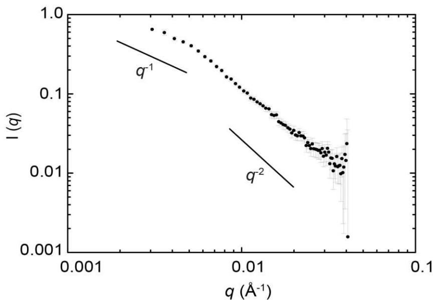
Figure S7. SANS pattern of an equimolar ( 1.0 \times 10^{-3} \text{ M} ) mixture of CB[8] and 3 in \text{D}_2\text{O} .
